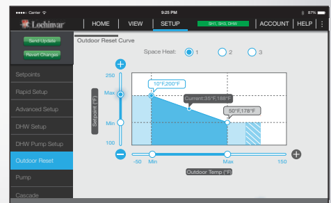
(CON-X-US displaying Reset Curve Graphing)
